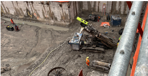
(Figure 2): Tieback installation, view of north east side.
