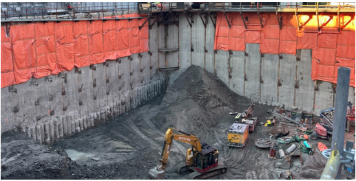
(Figure 3): Bulk excavation site progress, view of south west side.
