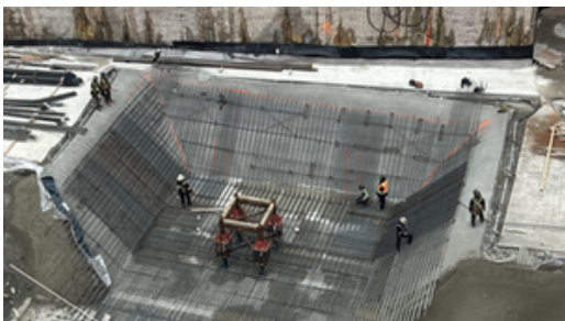
(Figure 3): Crane base progress, placing of steel
